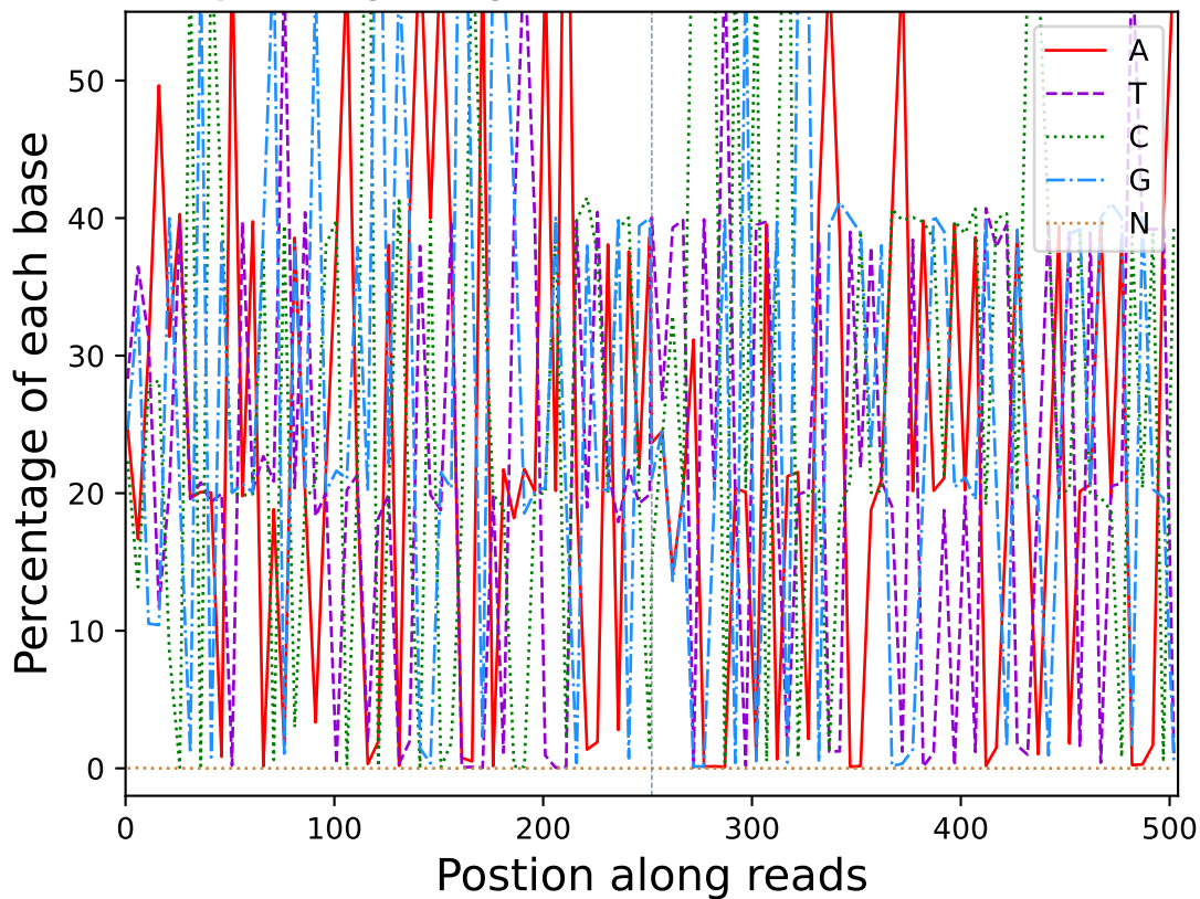
Base percentage along reads (R10810)
